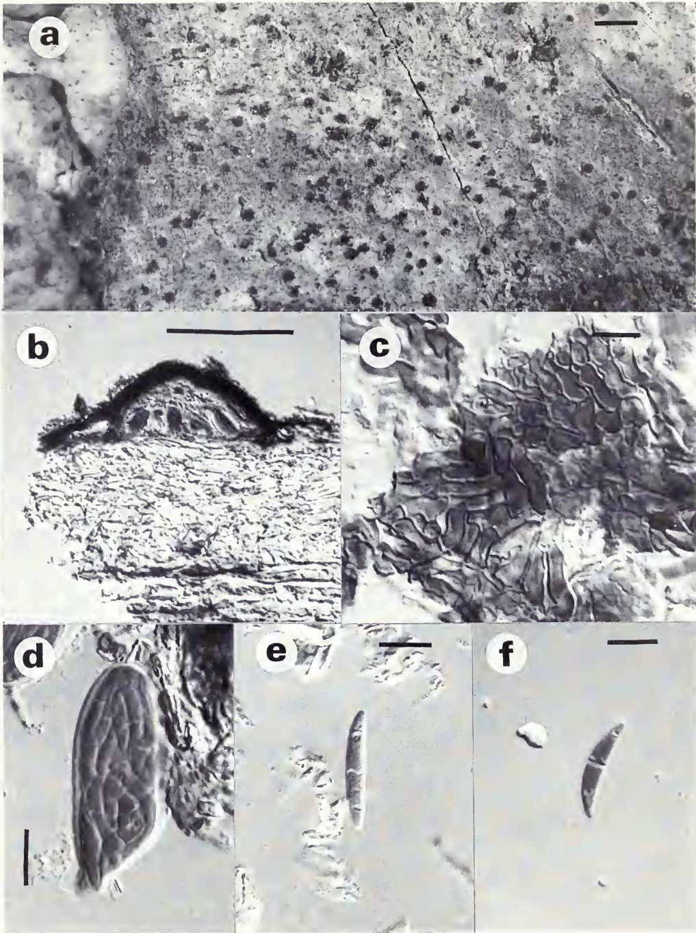
Fig. 20 Leptorhaphis tremulae Körber (L-lectotype) (a) Surface view; scale = 500 \mu\text{m} ; (b) Vertical section of ascoma; scale = 100 \mu\text{m} ; (c) Detail of involucrellum (surface view): textura epidermoidea-intricata; (d) 16-spored asci; (e), (f) Ascospores; scale = 10 \mu\text{m} .
